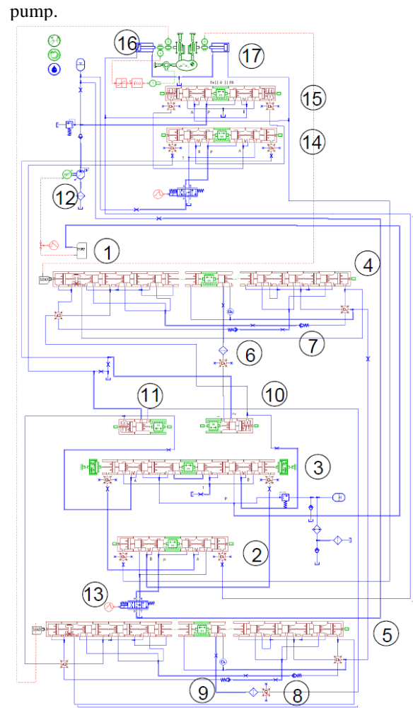
Fig. 3 Simulation model of concrete pump hydraulic system 1- the variable displacement pump 2、14-hydraulic pilot directional valve 3、15- main hydraulic directional valve 4、5-pumping cylinder 6、7、8、9-U-tube restrictor 10、11- pressure differential valve 12- constant pressure pump 13- electromagnetic directional valve、16、17-distributing cylinder
