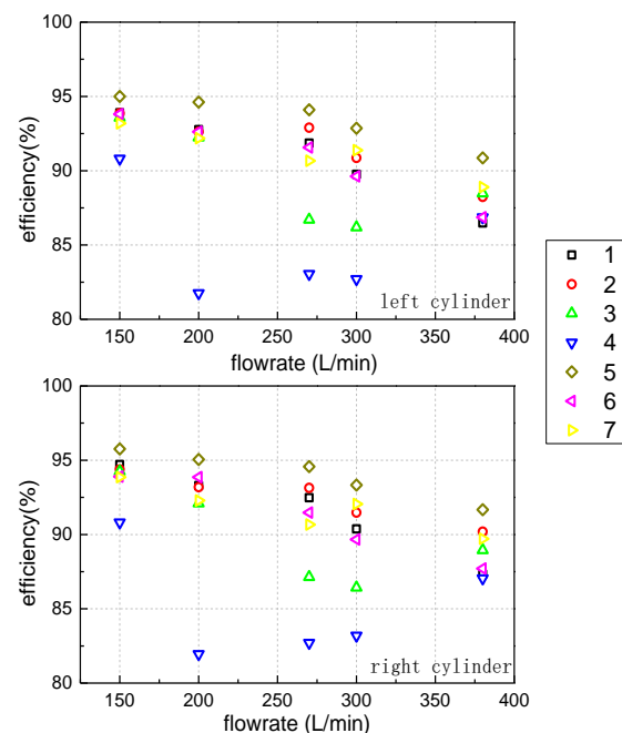
Fig. 13 Pumping efficiency
