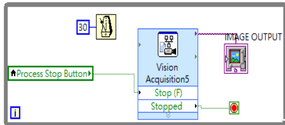
Fig. 9. The block-diagram of instant webcam control.
